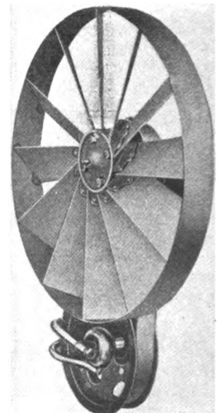
Fig. 15.—Example of the indiscriminate use of very many fan blades, a poor design.
